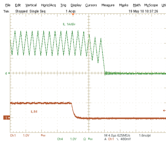
CH1: ILIM, 1V/div, CH4: inductor current, 1A/div, 4μs/div
