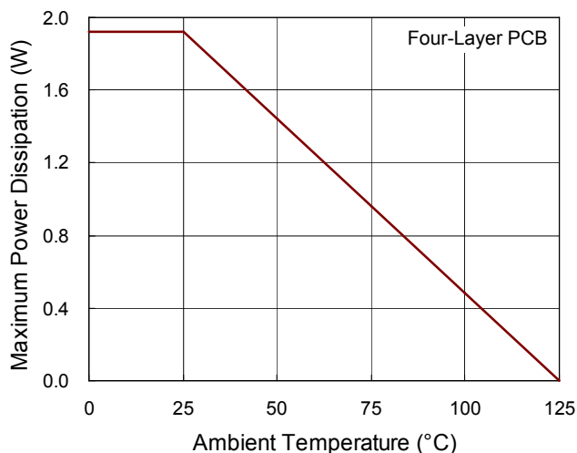
Figure 7. Derating Curve for the RT8205L/M Package
