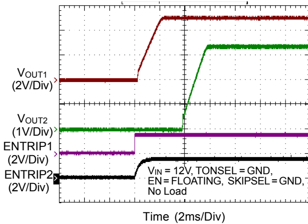
VOUT2 Delay-Start
