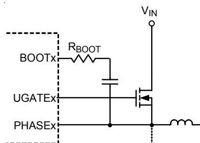
Figure 4. Reducing the UGATEx Rise Time
