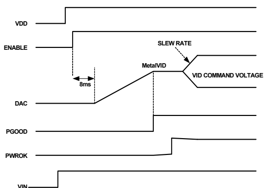
FIGURE 13. TYPICAL SOFT-START WAVEFORMS
