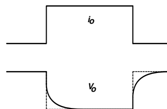
FIGURE 24. LOAD TRANSIENT RESPONSE WHEN C_n IS TOO LARGE
