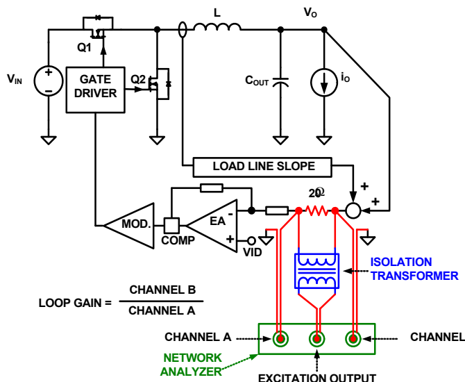
FIGURE 29. LOOP GAIN T1(s) MEASUREMENT SET UP
