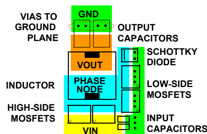
FIGURE 32. TYPICAL POWER COMPONENT PLACEMENT
