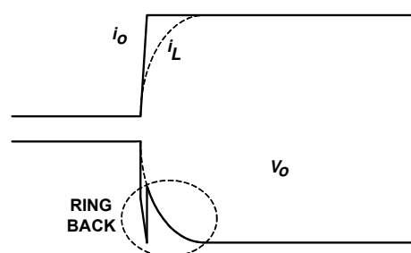
FIGURE 25. OUTPUT VOLTAGE RING-BACK PROBLEM
