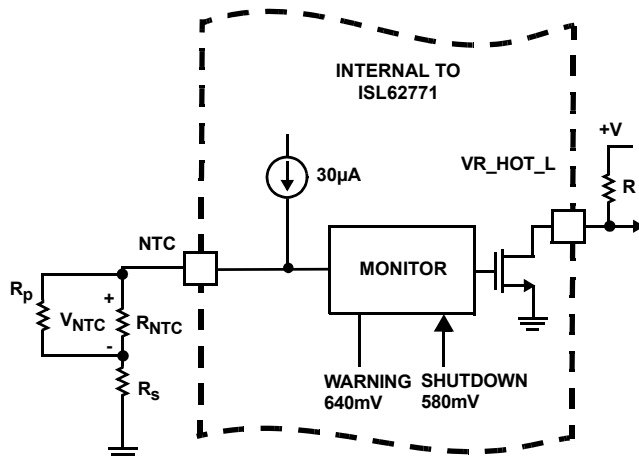
FIGURE 19. CIRCUITRY ASSOCIATED WITH THE THERMAL MONITOR FEATURE OF THE ISL62771
